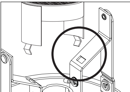
FOR USE WITH MR16, GU10, OR PAR20/PAR30
