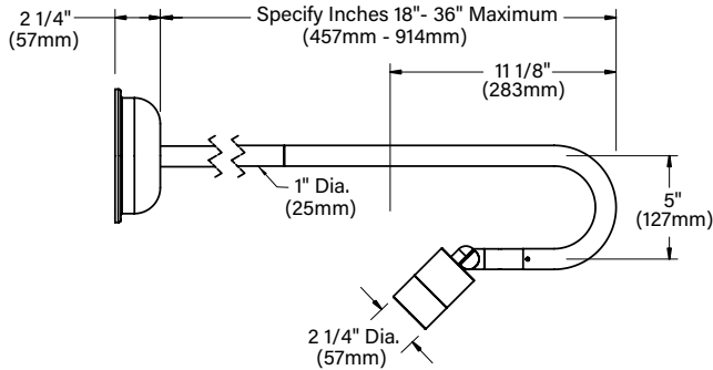
PC - SIDE VIEW
