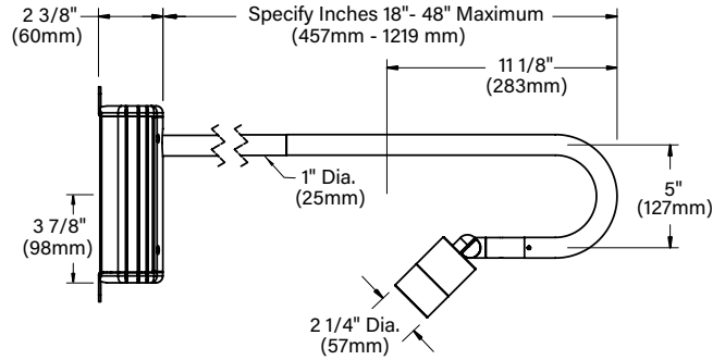
UPM - SIDE VIEW
