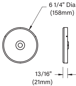
COVER DETAIL
