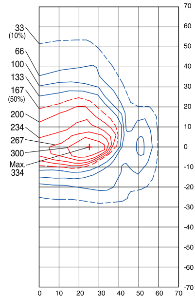
Wall Wash
