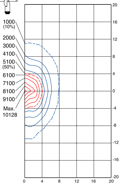
Spot
